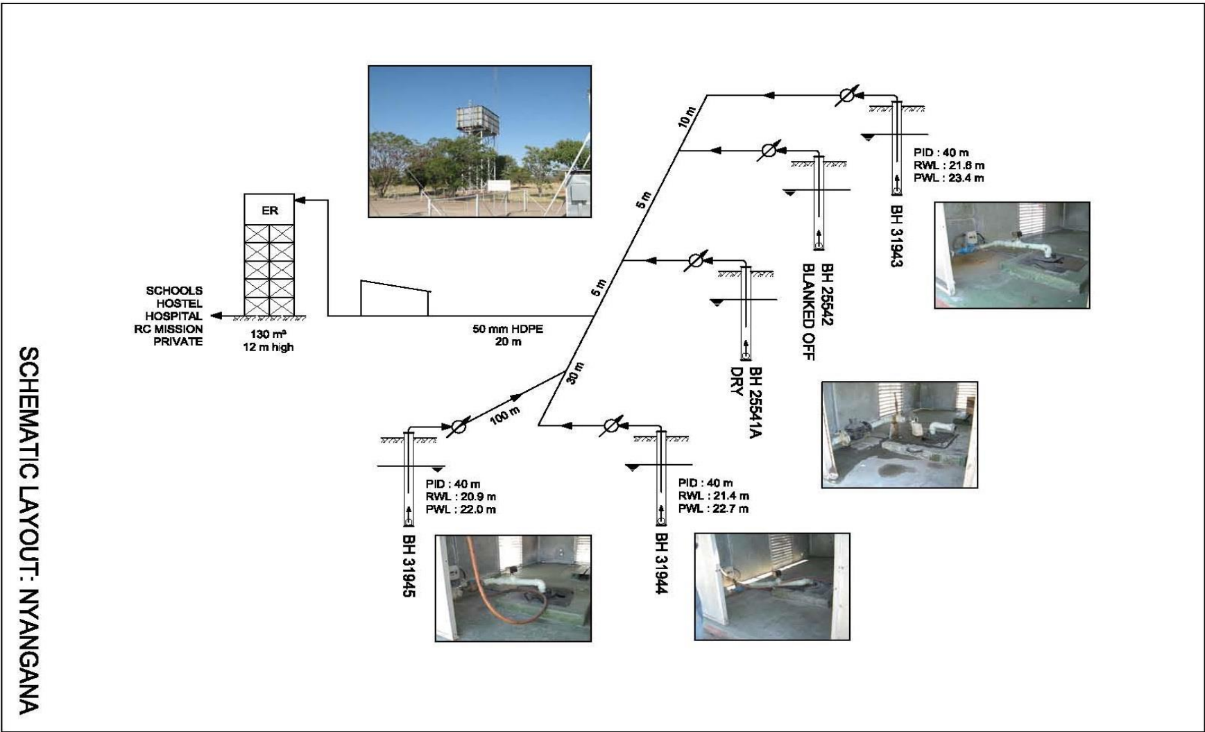
Figure 2: Nyangana Scheme Layout
