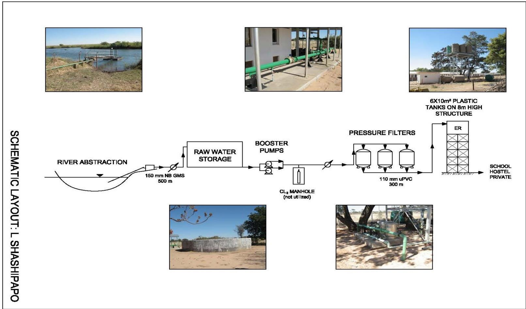
Figure 2: Linus Shashipapo Scheme Layout
